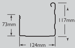
TRIMLINE
