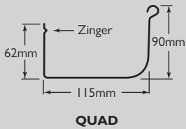
QUAD
