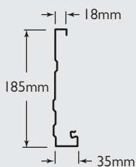
NOVALINE FASCIA
