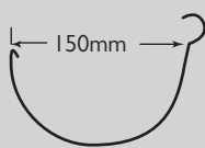
HALF ROUND
